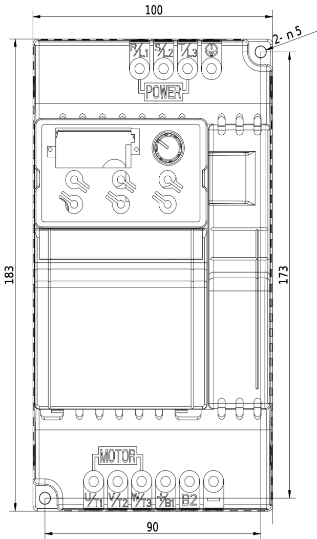
Dimensional drawing V800 - 3kW 4T0030
