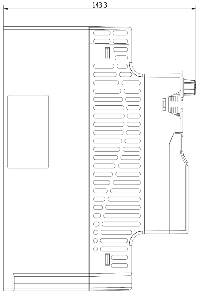
Dimensional drawing V800 - 3kW 4T0030
