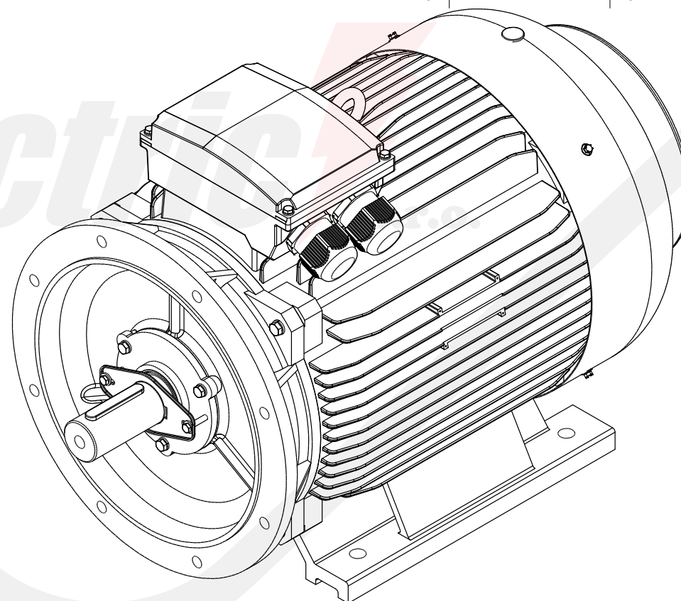
3LC-280M-B35 Mounting diagram
