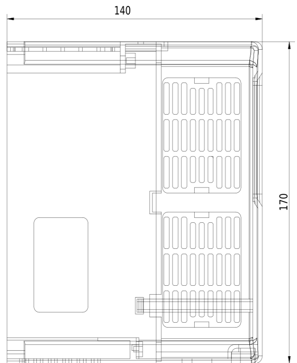
Dimensional drawing V810 - 0,4kW 4T0004
